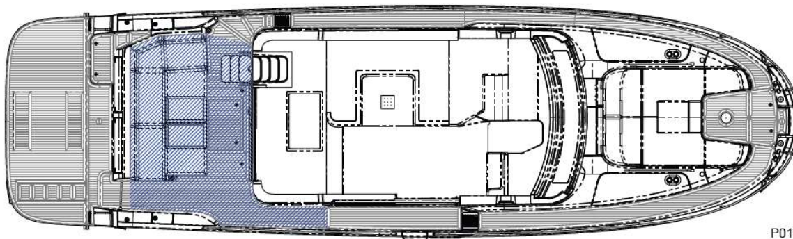
AREA AFT DECK 8,5 M2
